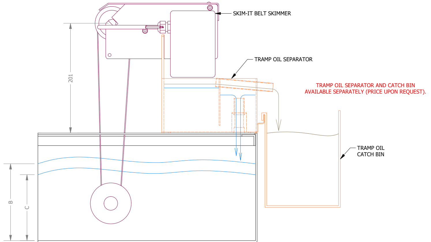
TANK SHOWN WITH SKIM-IT BELT SKIMMER FOR REFERENCE
